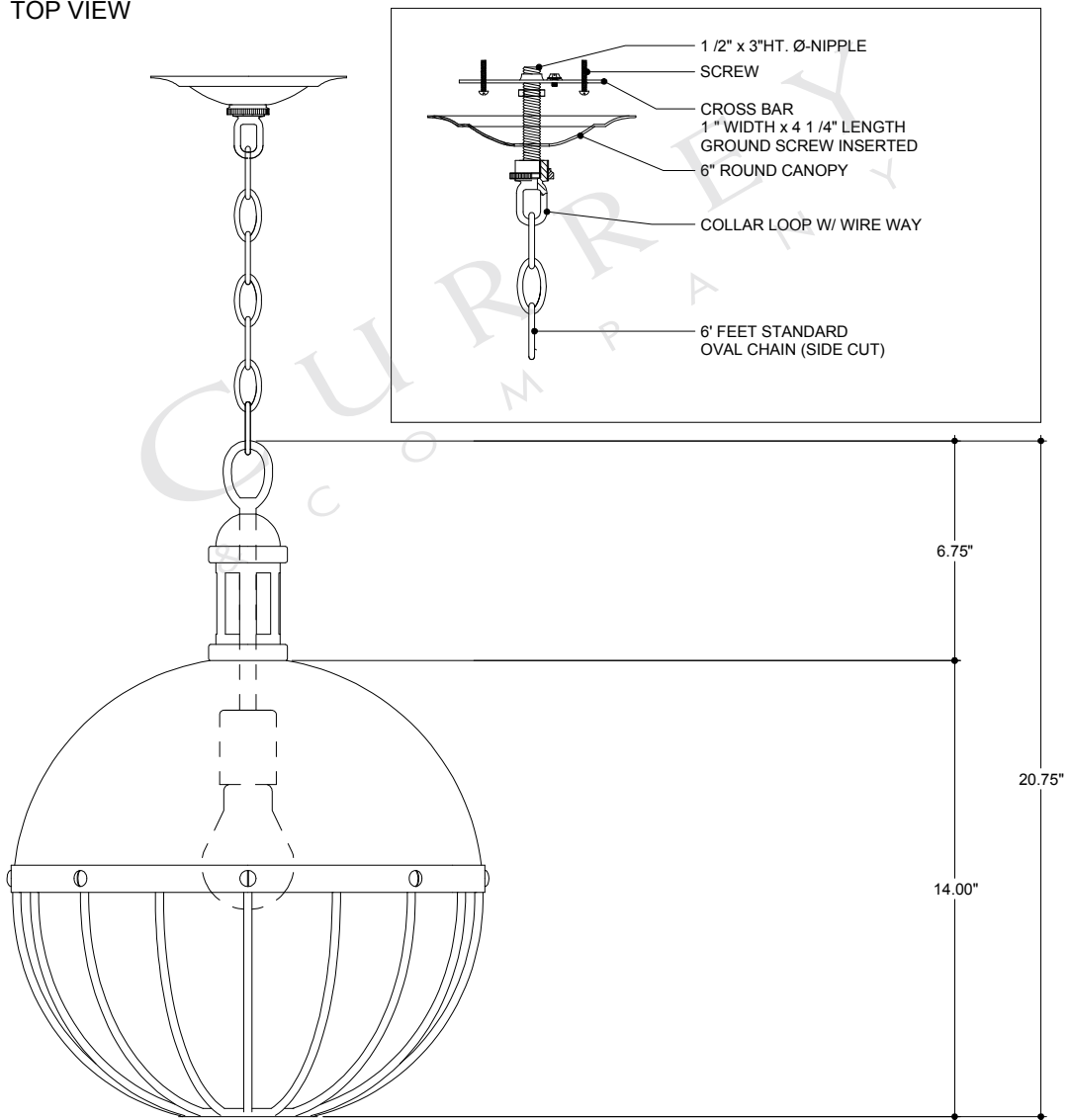
FRONT VIEW
