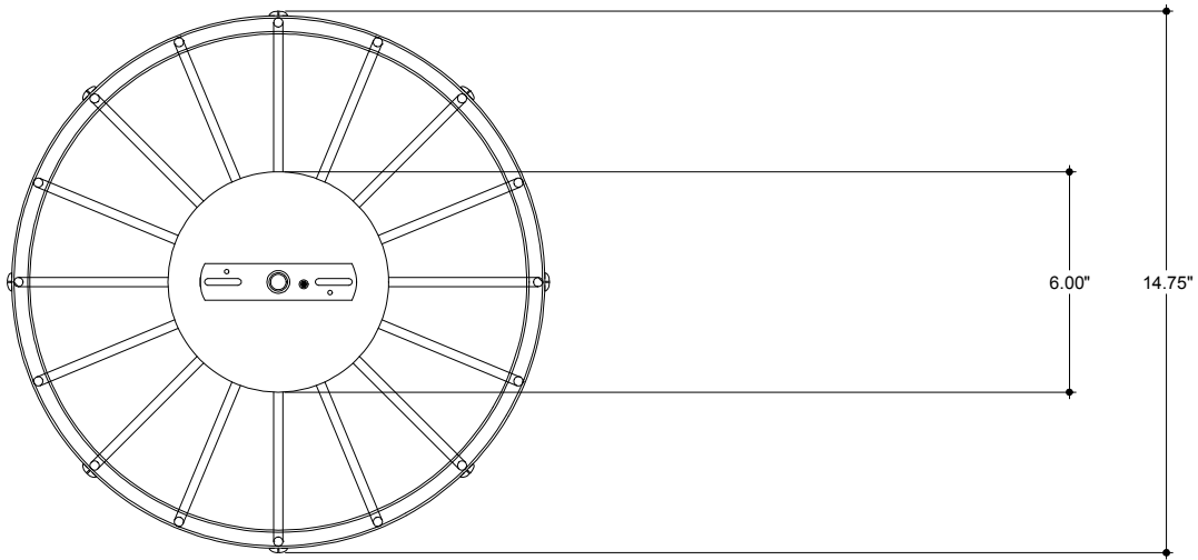
TOP VIEW
