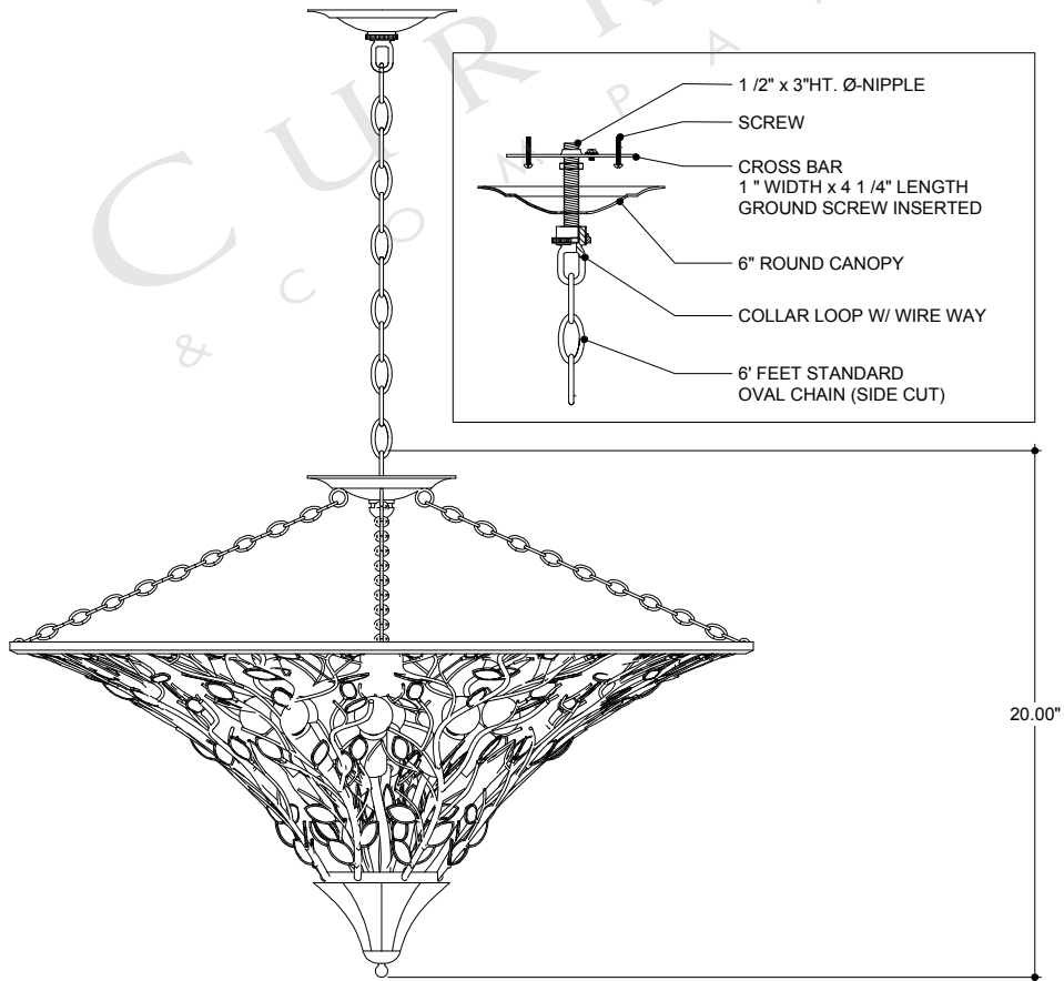
FRONT VIEW
