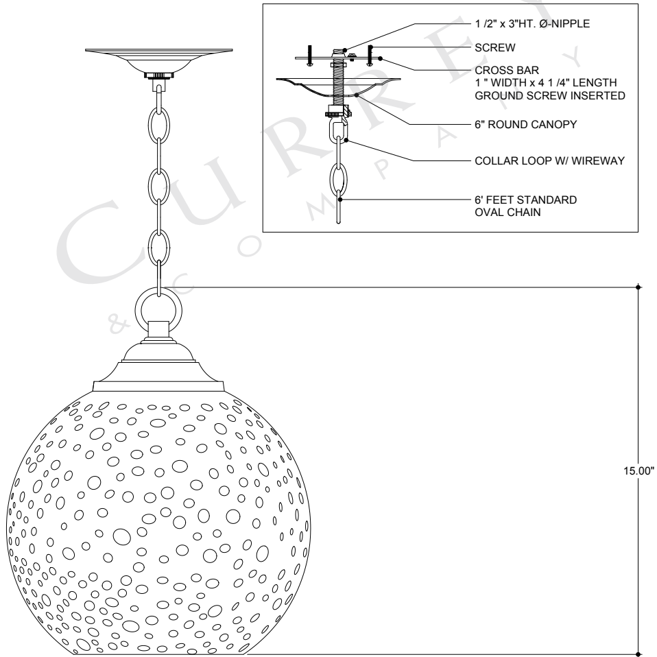
FRONT VIEW
