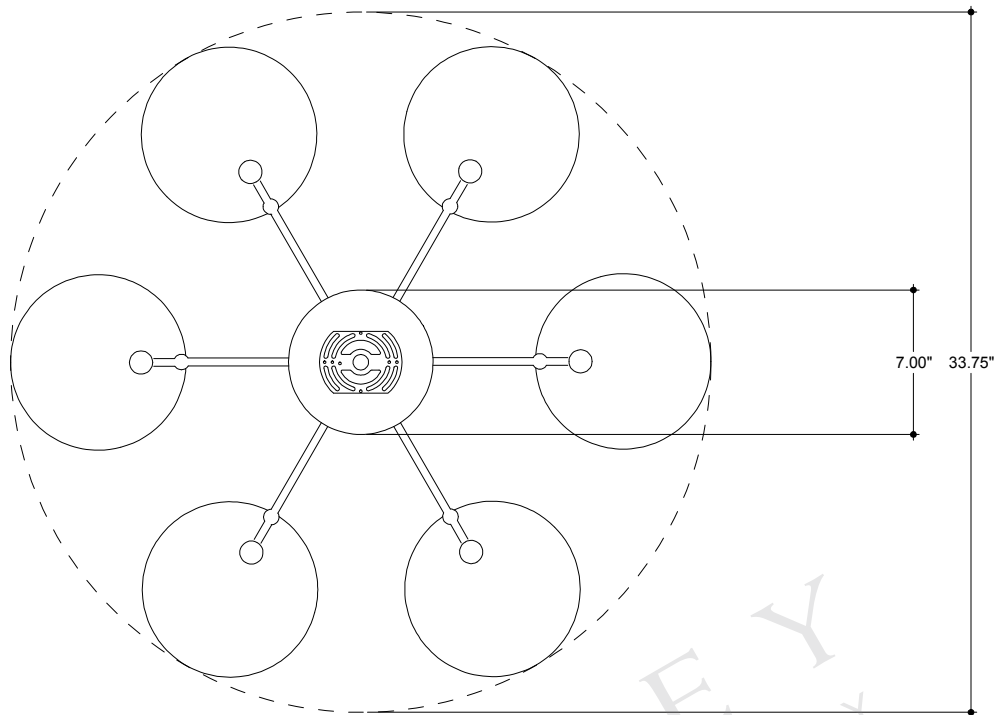
TOP VIEW
