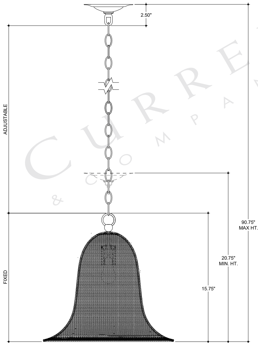
FRONT VIEW
