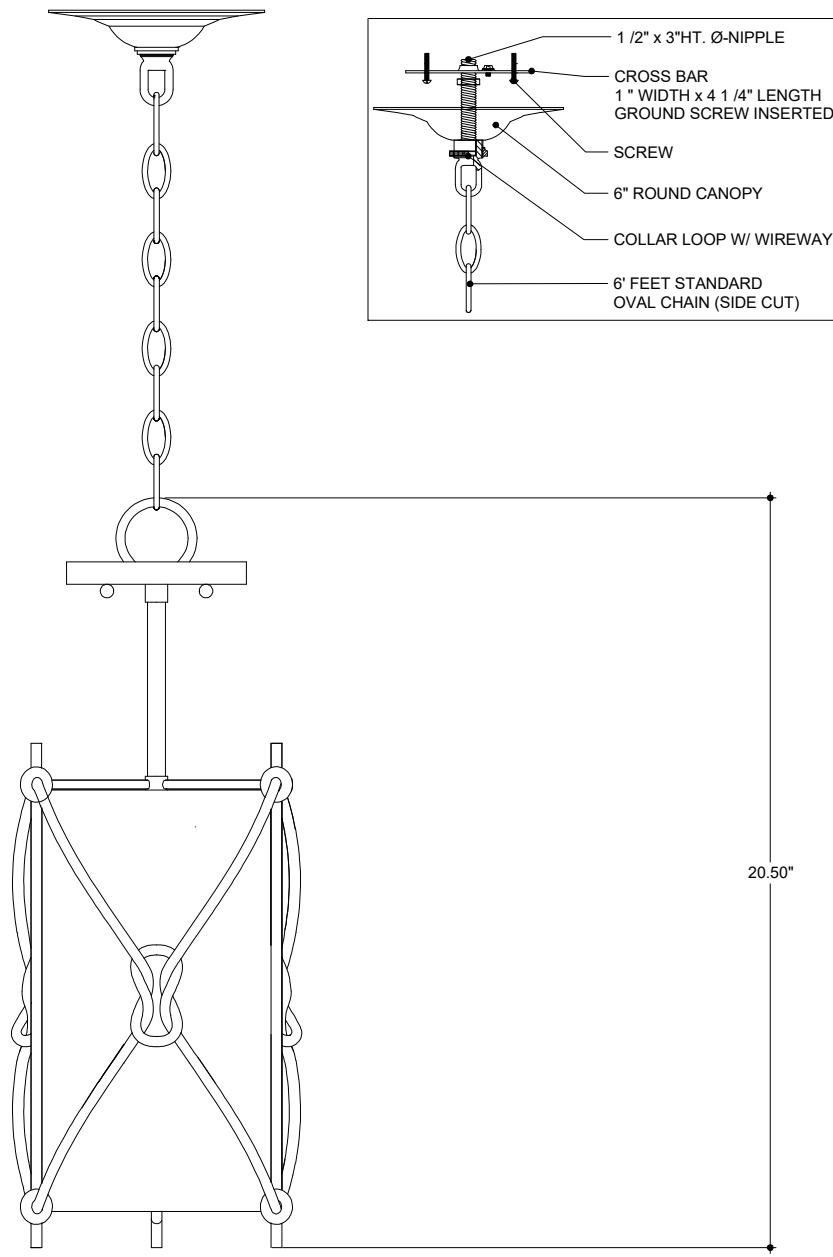
FRONT VIEW
