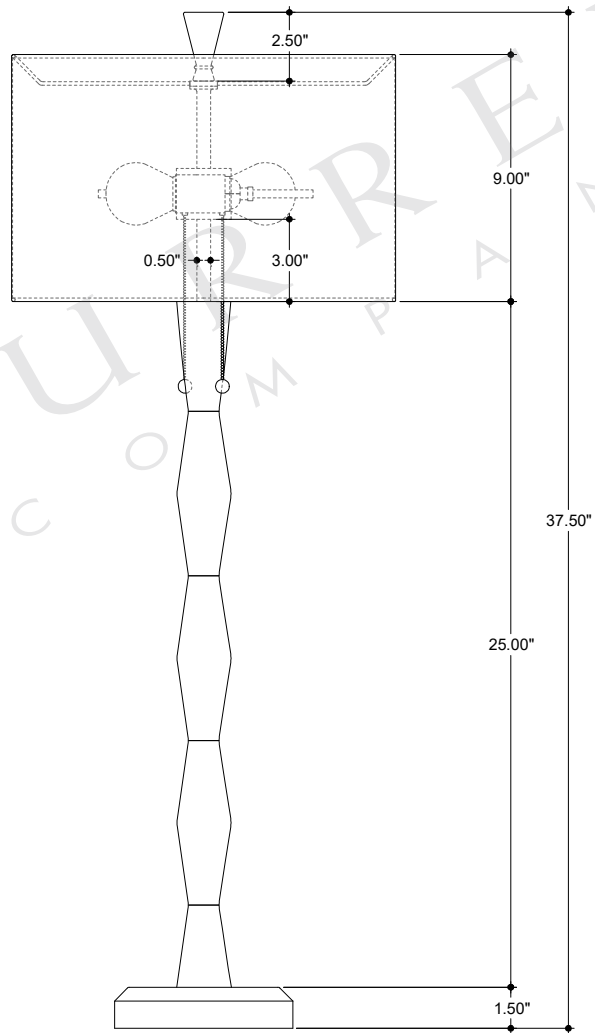
FRONT VIEW
