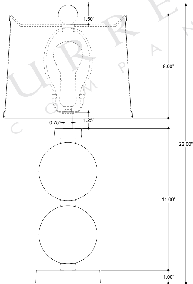
FRONT VIEW
