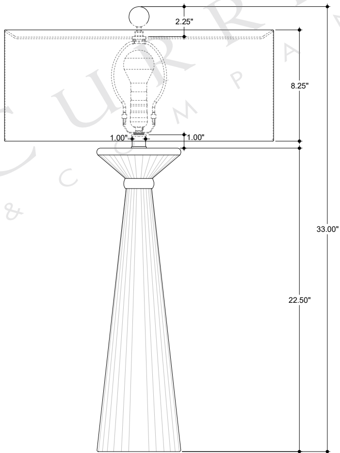
FRONT VIEW
