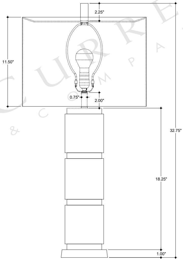
FRONT VIEW
