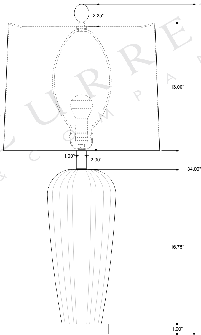
FRONT VIEW
