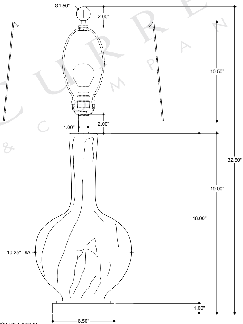
FRONT VIEW
