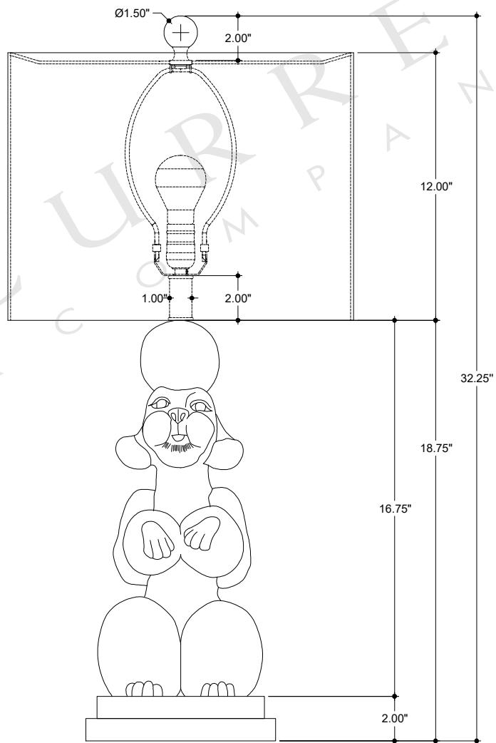
FRONT VIEW
