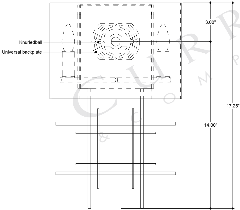
FRONT VIEW
