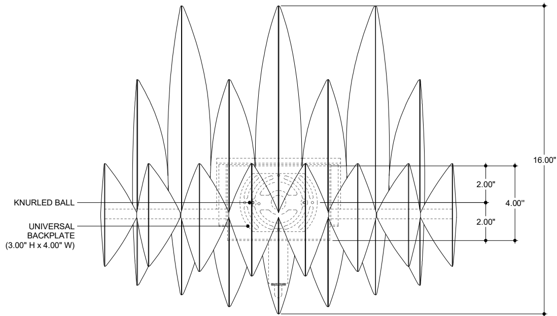
FRONT VIEW
