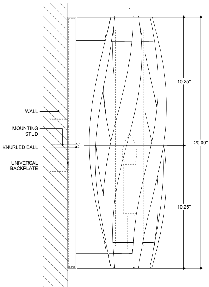
SIDE VIEW
