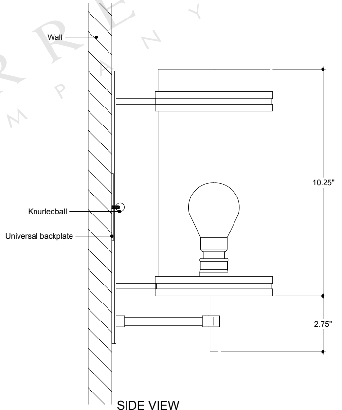
SIDE VIEW
