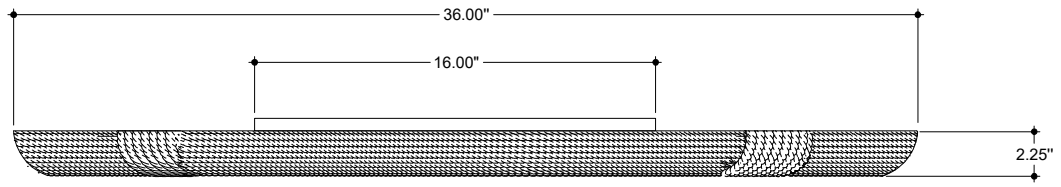
TOP VIEW
